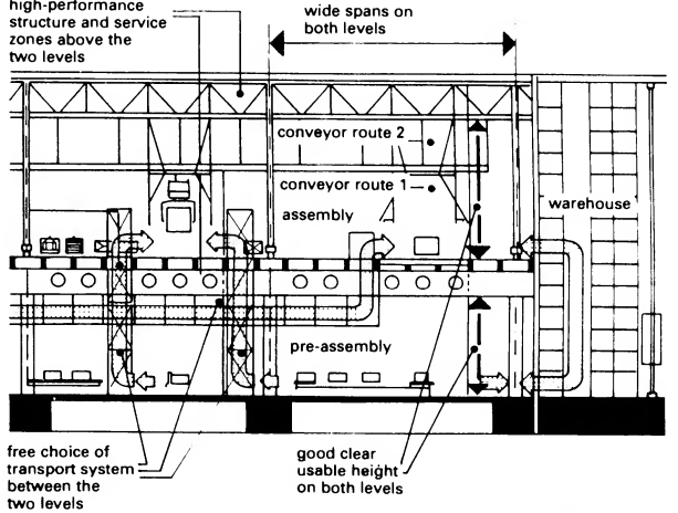
5 Example of a production store integrated into the assembly
